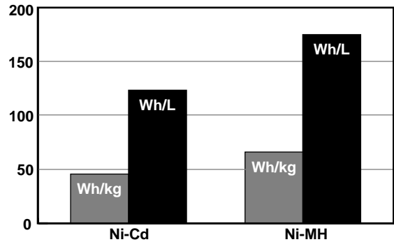
Gravimetric and volumetric energy density of Ni-Cd and Ni-MH cells.
