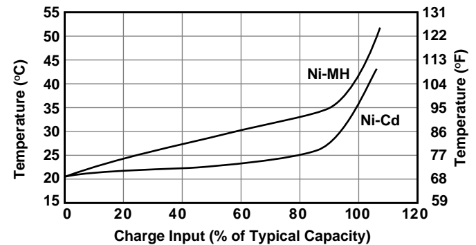
Typical charge temperature characteristics of Ni-MH and Ni-Cd batteries.
