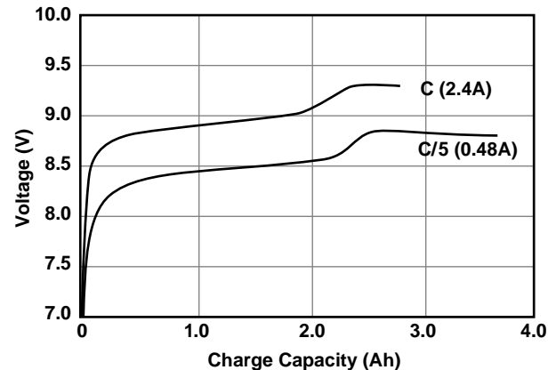
Charge voltage of DURACELL DR30 Ni-MH batteries at various rates.
