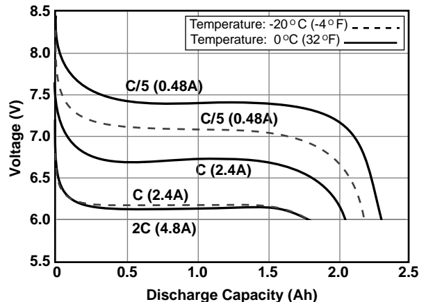
Voltage and capacity of DURACELL DR30 Ni-MH batteries at various discharge temperatures and rates.
