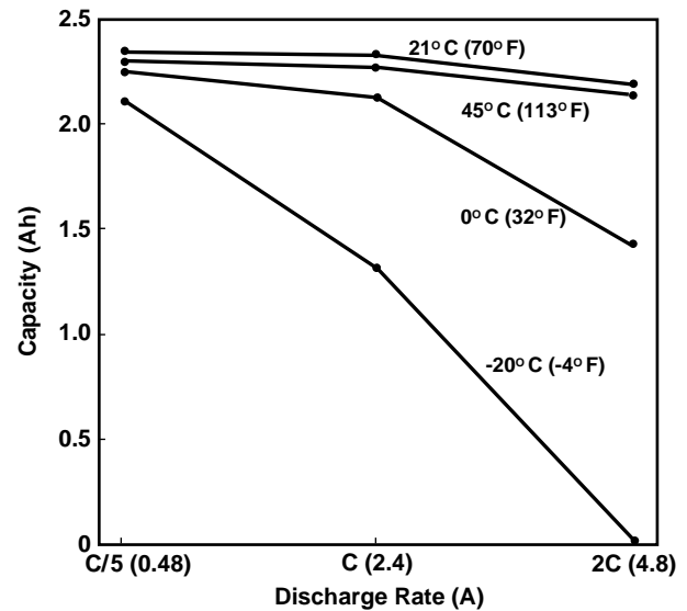
Typical capacity of DURACELL DR30 batteries under constant current discharges at various temperatures.
