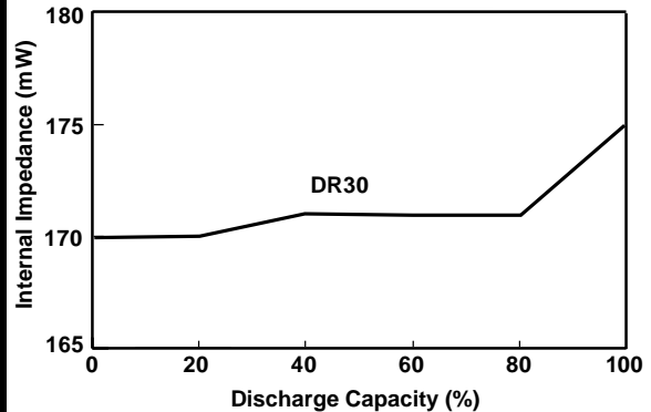
Internal impedance of DURACELL DR30 Ni-MH batteries at various discharge capacities.
