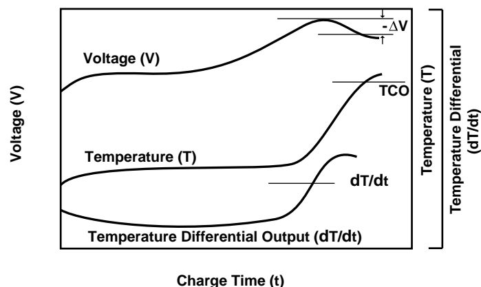
Charge characteristics of Ni-MH batteries using various charge termination methods.
