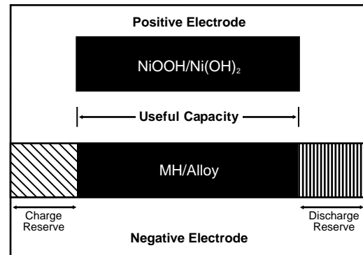
Schematic representation of the electrodes, divided into useful capacity, charge reserve and discharge reserve.
