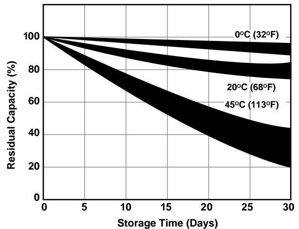
Self-discharge characteristic of Ni-MH cells at various temperatures.
