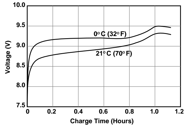
Charge voltage of DURACELL DR30 Ni-MH batteries at various temperatures.
