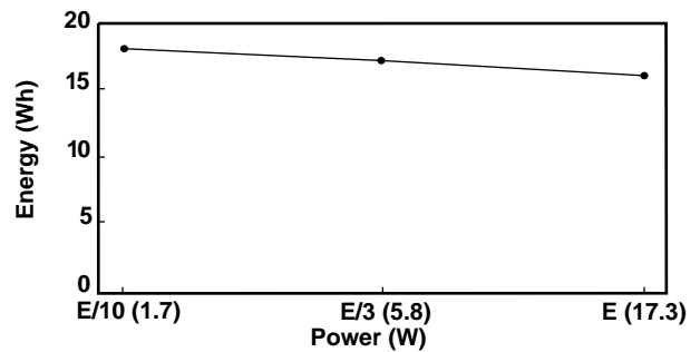
Typical energy of DURACELL DR30 batteries under constant power discharges.
